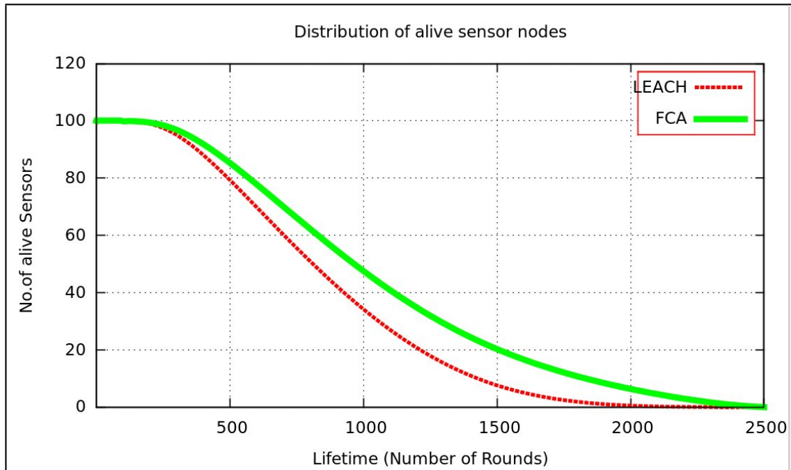
Fig. 6. Scenario 1: Distribution of alive sensor nodes according to the number of rounds for each algorithm
