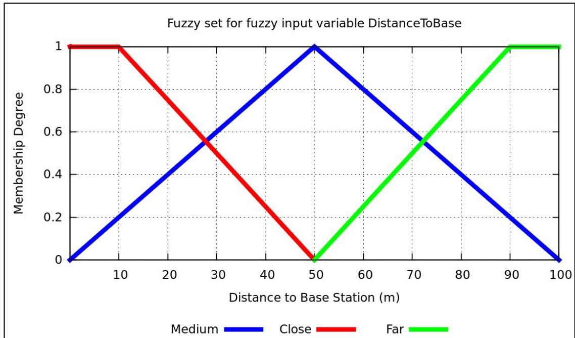
Fig. 3. Fuzzy set for fuzzy input variable DistanceToBase
