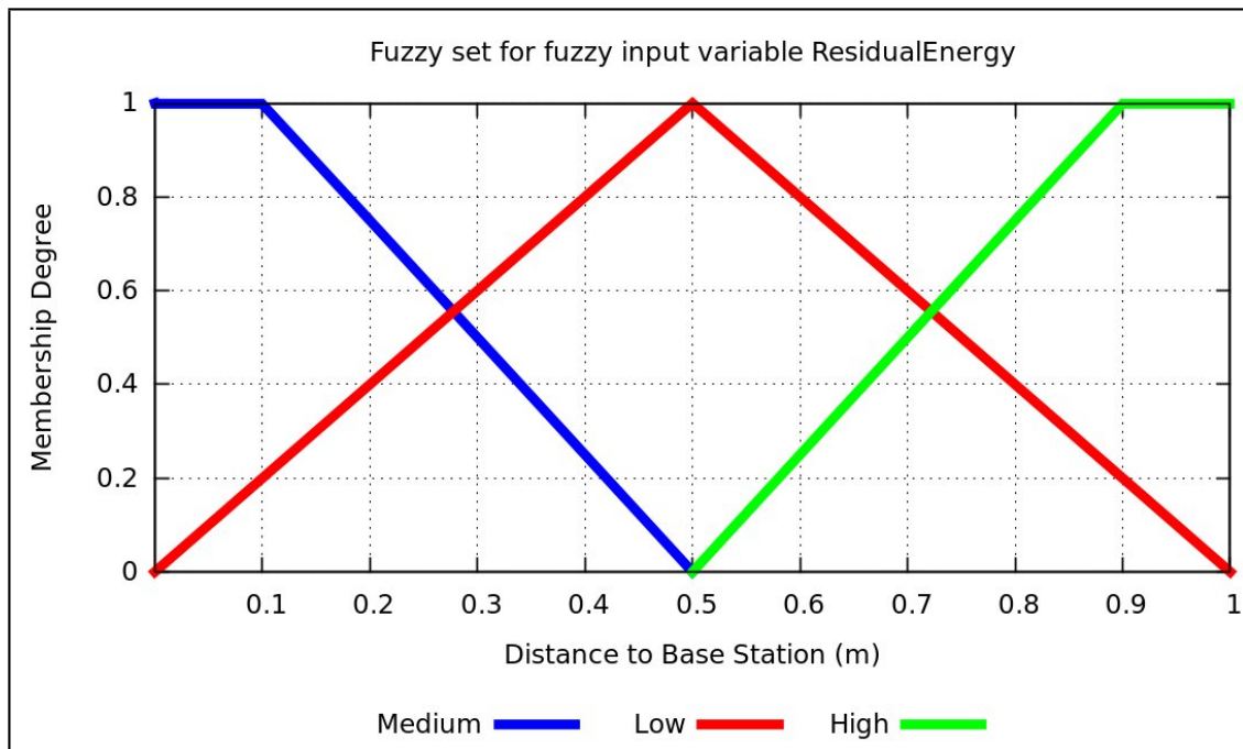
Fig. 4. Fuzzy set for fuzzy input variable ResidualEnergy
