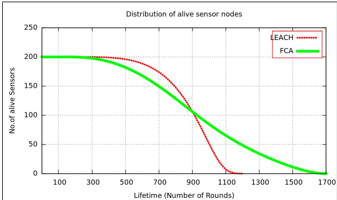
Fig. 8. Scenario 2: Distribution of alive sensor nodes according to the number of rounds for each algorithm
